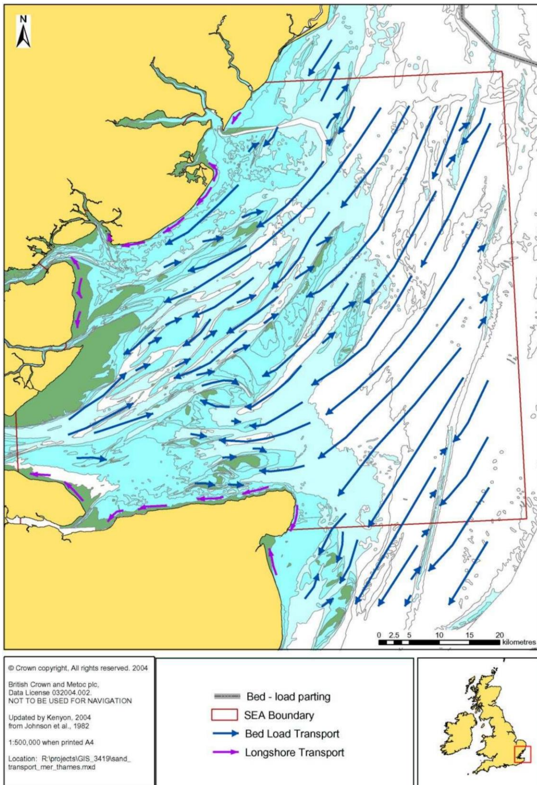
Plate 1.22 Map of net sand transport paths in the Outer Thames Estuary (Kenyon & Cooper, 2005).
