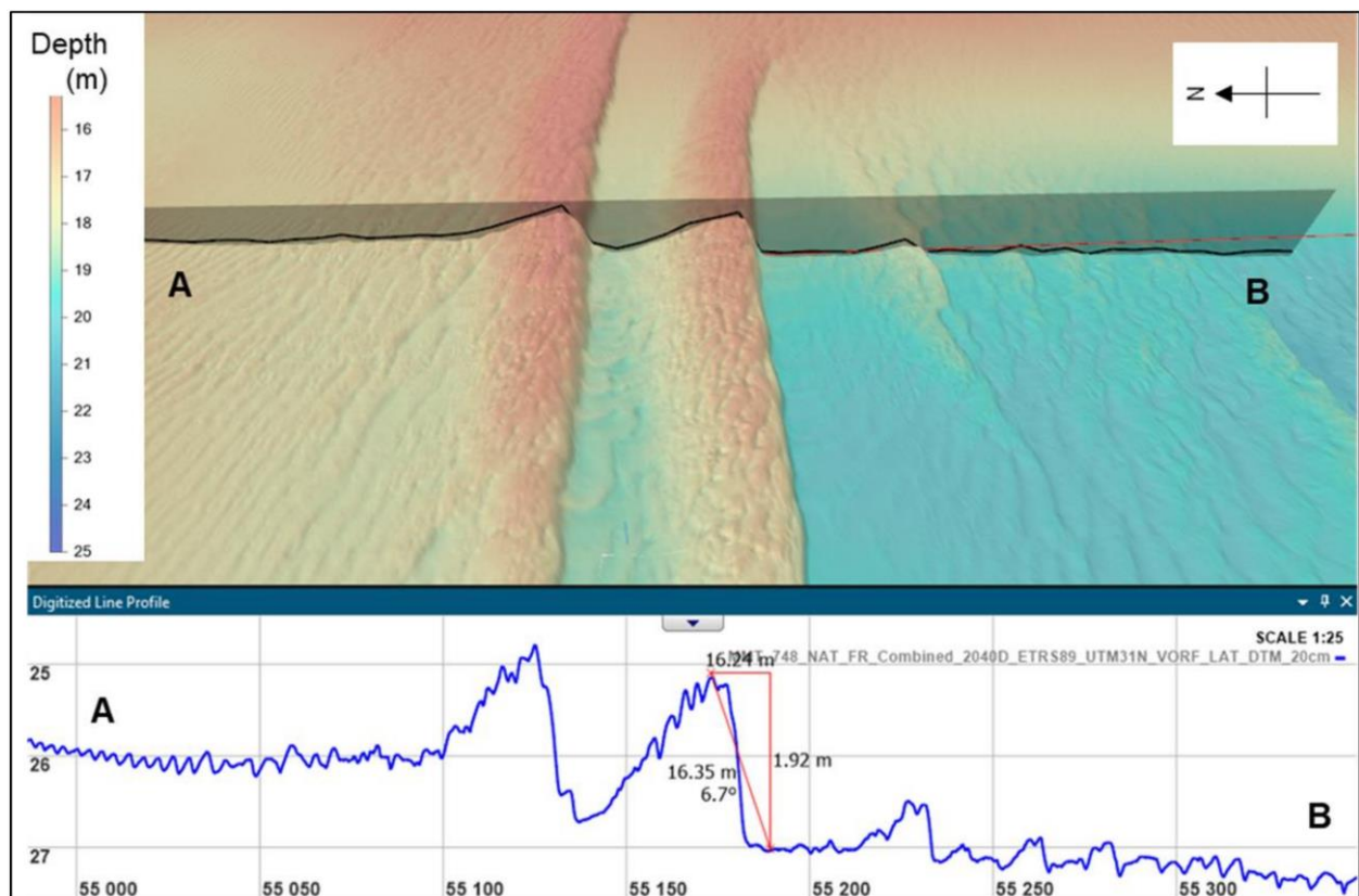
Plate 1.32 2 m high megaripples on the route at KP 50.5 (MMT, 2022).
