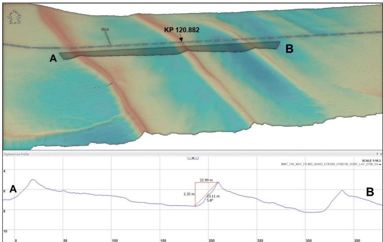
Plate 1.26 Bedforms along the route associated with mega ripple stoss slopes, example shown at KP120.882 (MMT, 2022).
