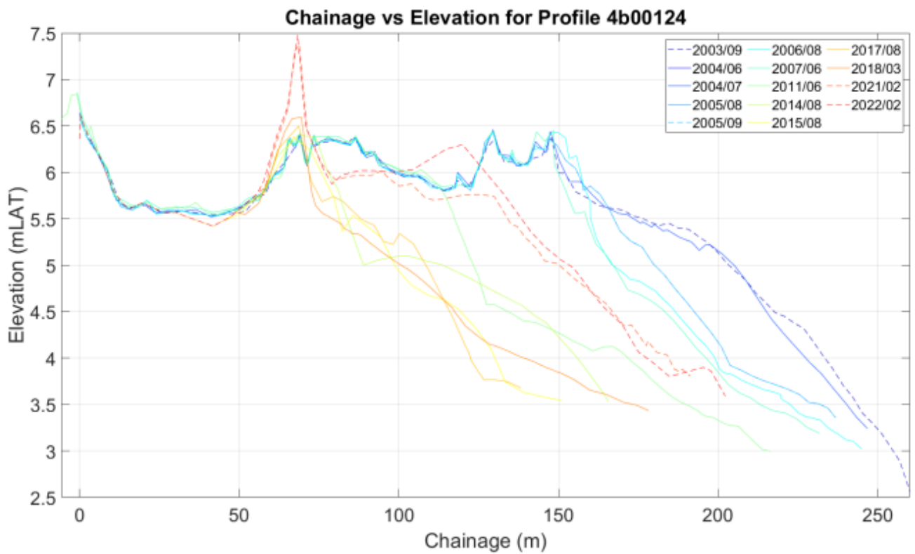
Plate 1.24. Profile 4b000124 elevation change (ABPmer, 2024b)
