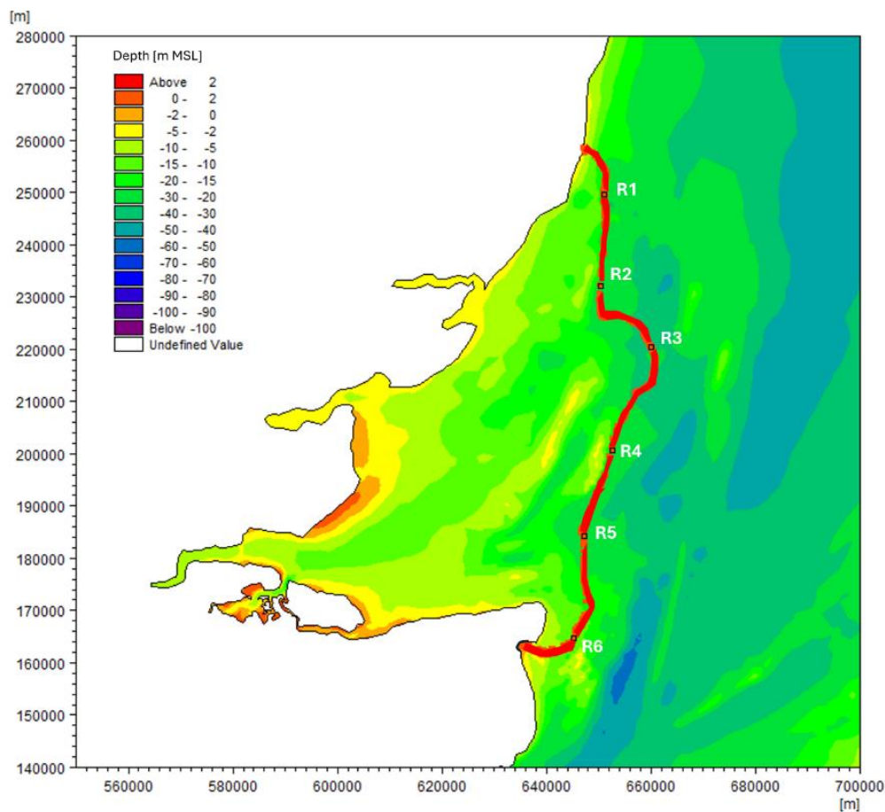
Plate 1.36 Hydrodynamic model bathymetry showing the Offshore Scheme Boundary (red line) and 6 sediment release locations
