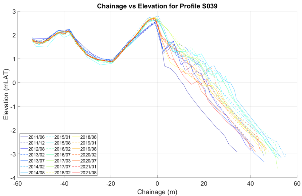
Plate 1.16 Profile changes 2011-2021 – Profile S039 (ABPmer, 2024a)
