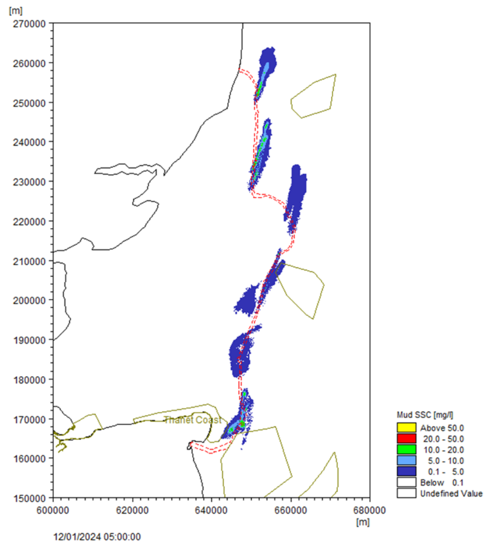
Plate 1.37 Mud SSC levels for jetting installation commencing on spring tides with output on flood (left) and ebb (right) tide after first 24 hours of activity
