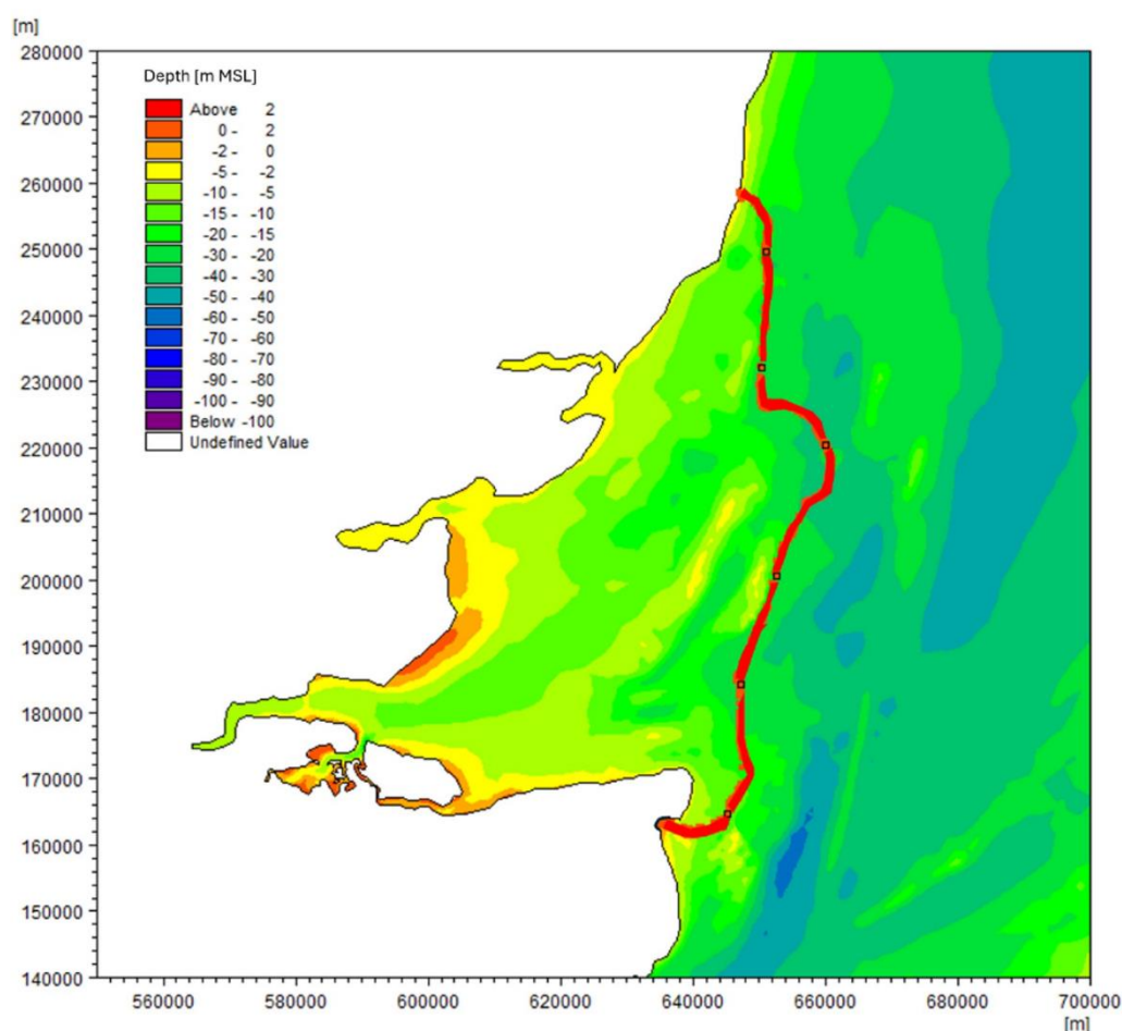
Plate 1.28 Water depth (m MSL)
