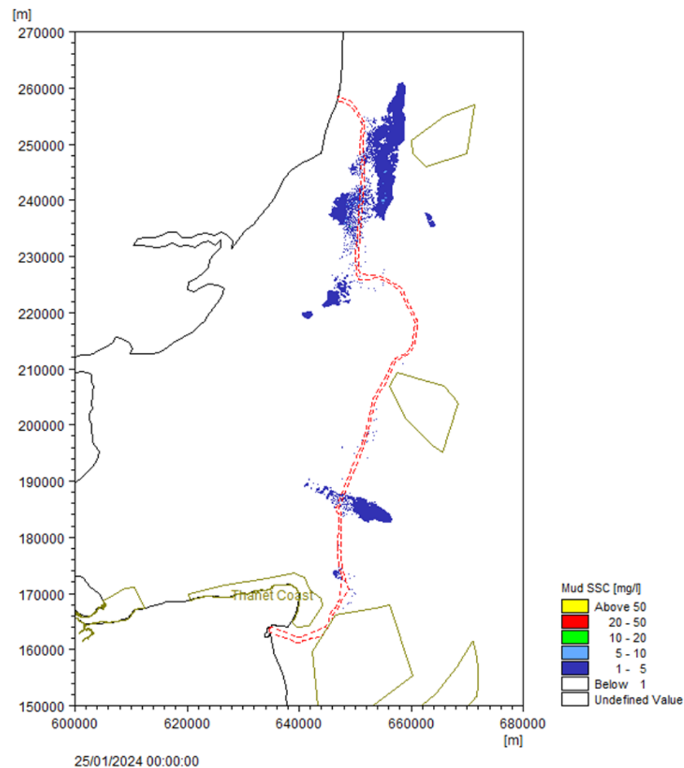
Plate 1.38 Mud SSC levels for jetting installation commencing on spring tides with output at +7 days (left) and +14 days (right) after start of activity
