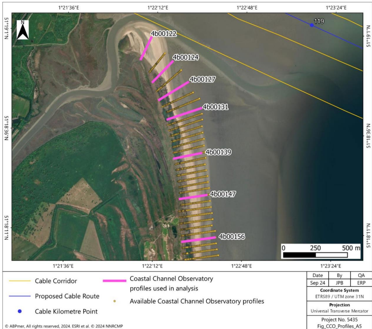
Plate 1.23 Location of topographic profiles available (in yellow) and selected for analysis (in pink) (ABPmer, 2024b).
