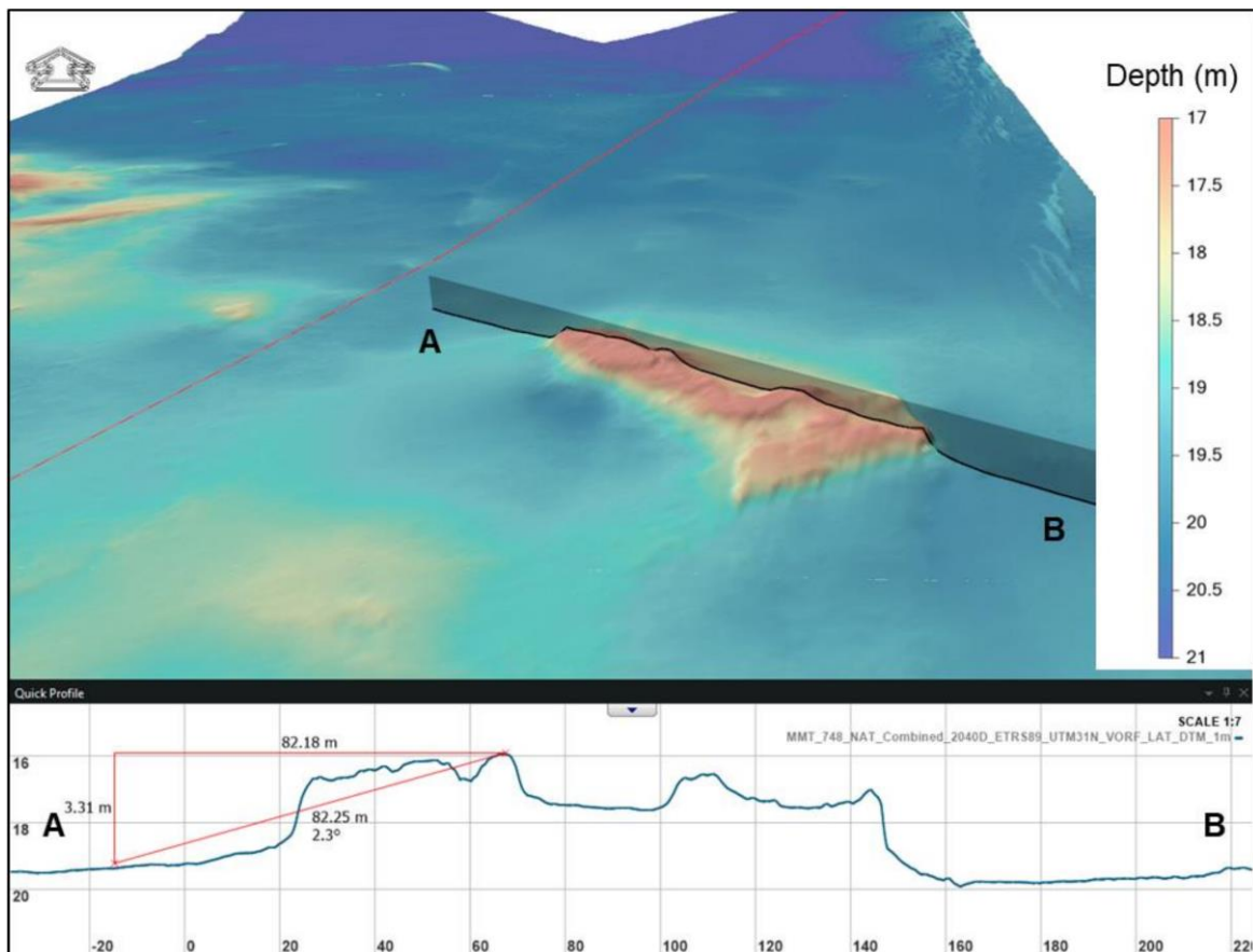
Plate 1.29 Outcrop at KP 8 with a height of 3.3 m above the surrounding seafloor (MMT, 2022).
