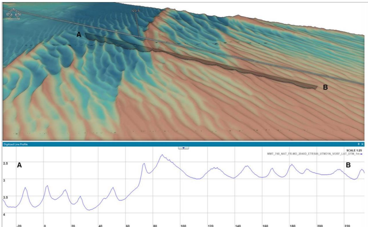
Plate 1.27 Bedforms along the route associated with lee slopes of a mega ripple area at KP 123.475 (MMT, 2022).
