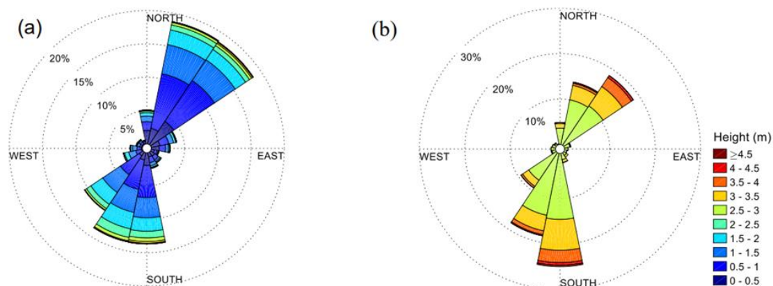
Plate 1.2. From Atkinson and Esteves (Atkinson & Esteves, 2019) – West Gabbard buoy wave roses for (a) all waves and (b) waves of H_s > 2.5 m, showing the percentage of waves of different heights ( H_s ) that approach from different directions in the period June 2006 to March 2018 (168685 records, 98% data coverage).
