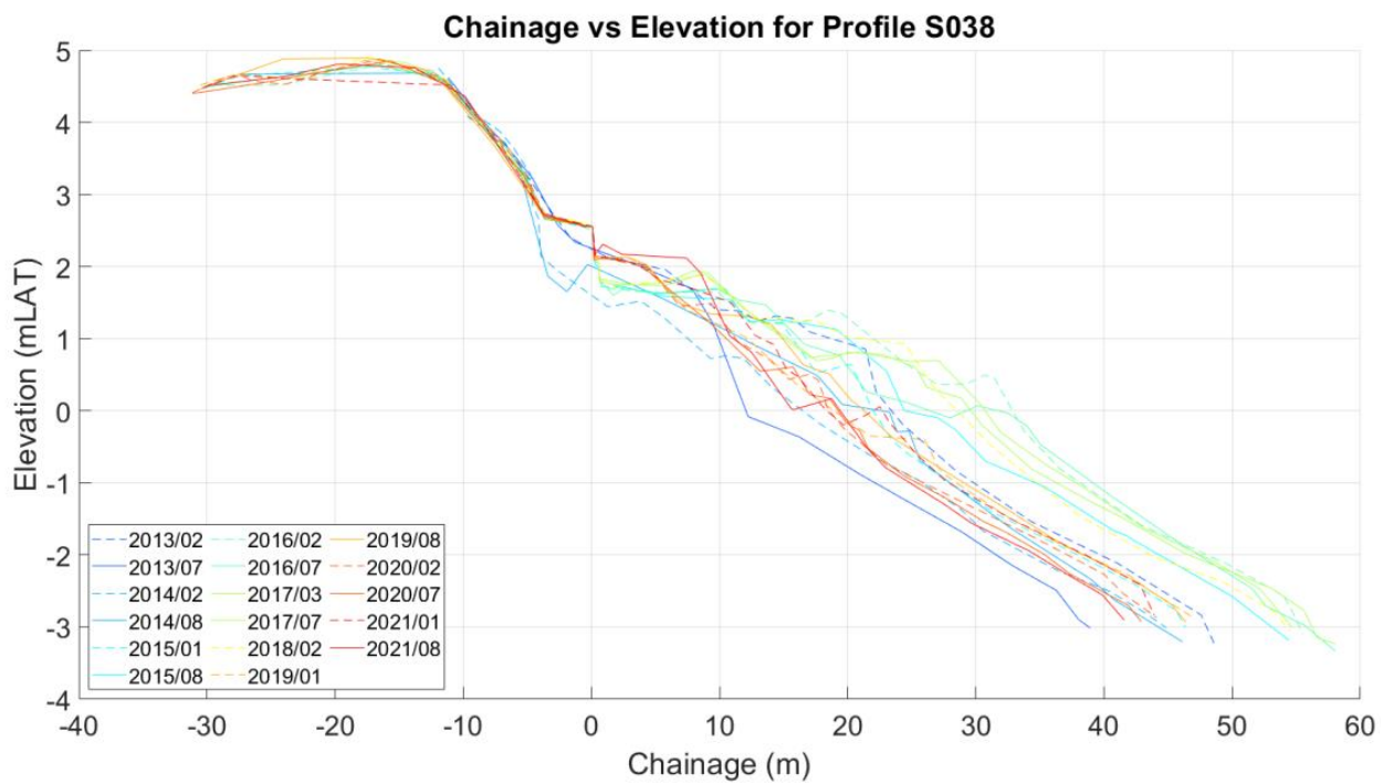
Plate 1.15 Profile changes 2013-2021 – Profile S038 (ABPmer, 2024a)
