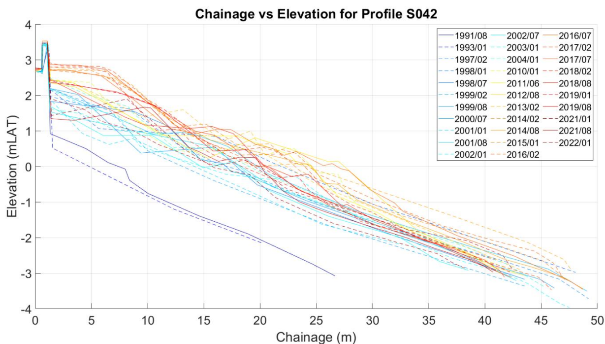
Plate 1.19 Profile changes 2013-2021 – Profile S042 (ABPmer, 2024a)
