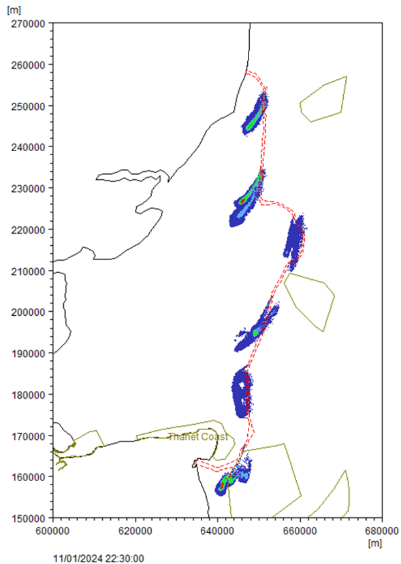
Plate 1.37 Mud SSC levels for jetting installation commencing on spring tides with output on flood (left) and ebb (right) tide after first 24 hours of activity
