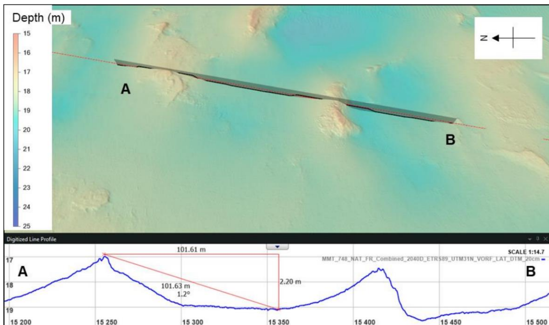
Plate 1.30 A profile along the route between KP 10 and KP 10.5 over a sample of the outcrops in the area. The outcrops stand >2 m above the surrounding seabed (MMT, 2022).
